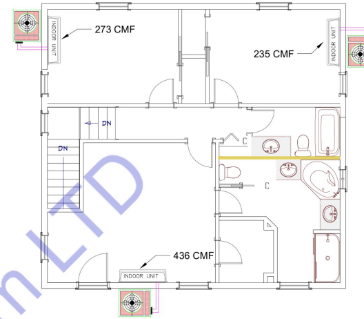
HVAC PLAN 2ND FLOOR
