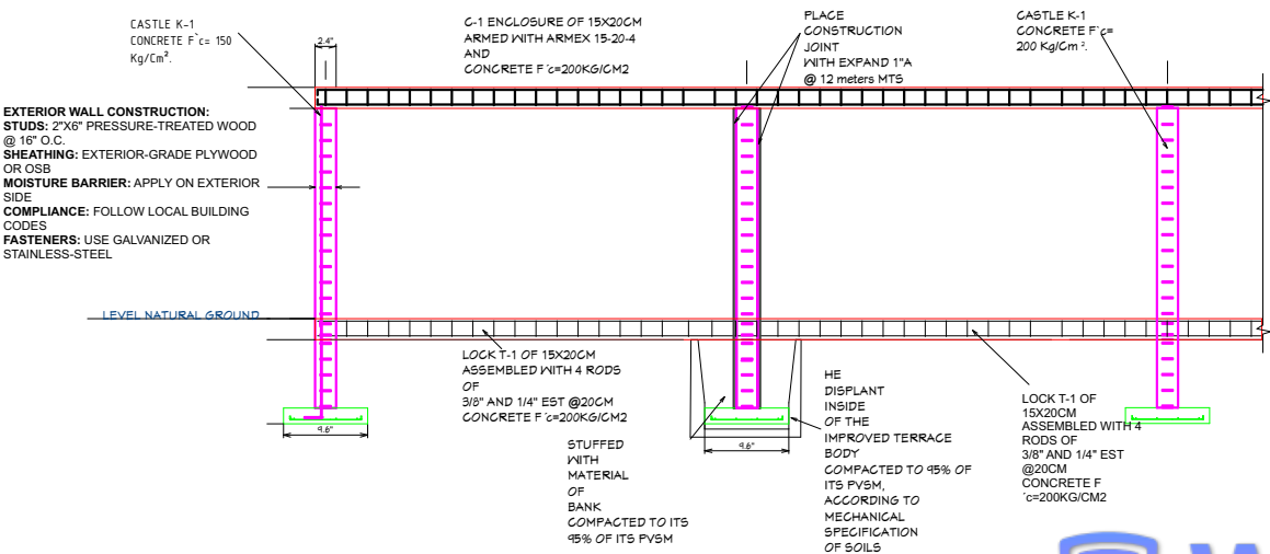
Concrite Wall Detail
