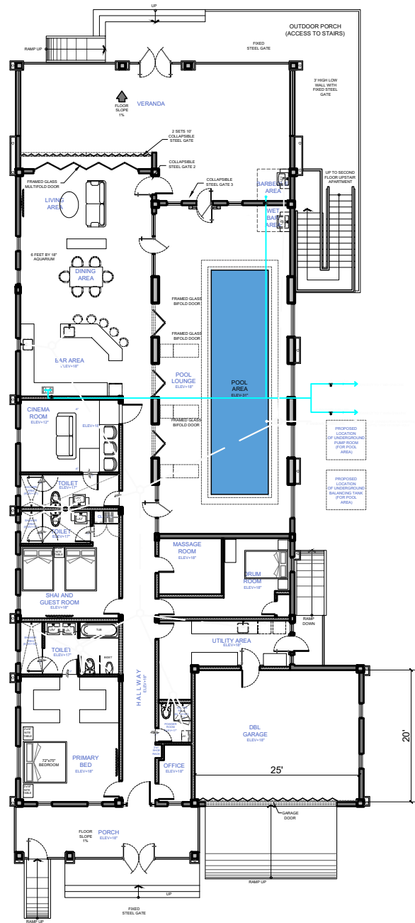
1 GROUND FLOOR PLAN AS-BUILT SCALE: 1:5
