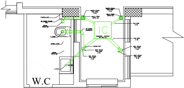
Ground Floor Plan SCALE 1:50
