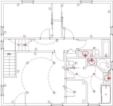
LIGHTING & OUTLET PLAN 2ND FLOOR
