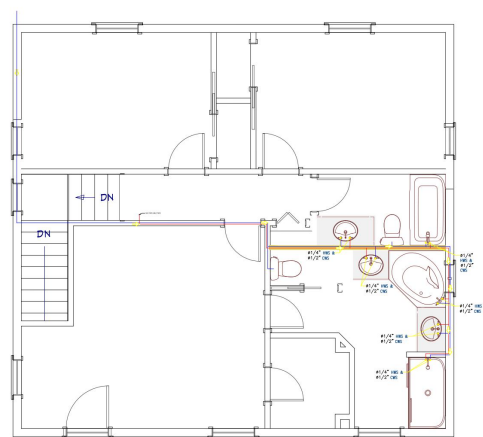
WATER SUPPLY PLAN 2ND FLOOR
