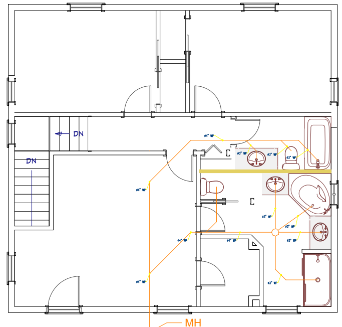
GAS & SEWERAGE LINE PLAN 2ND FLOOR
